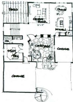
FIRST FLOOR PLAN 1106 sq' THAT 1047 sq'
